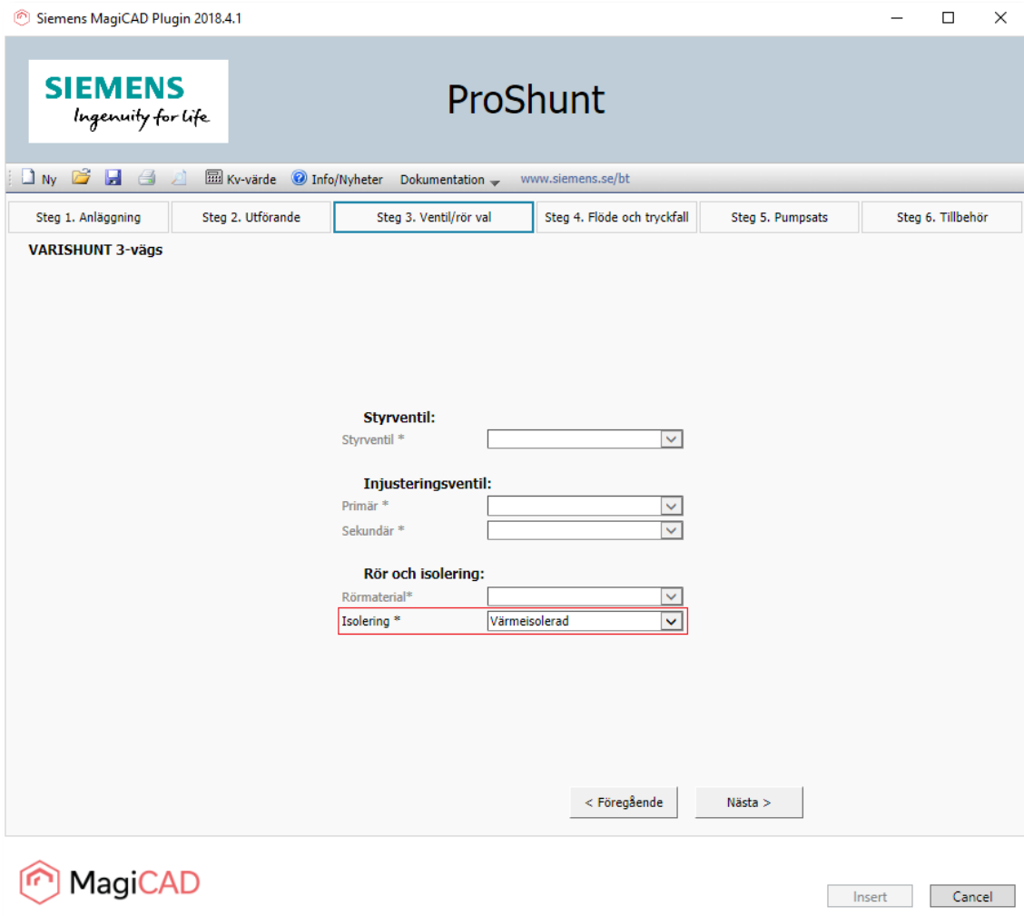
Figure 6 Step 3/6 – VARISHUNT unit isolation selection
