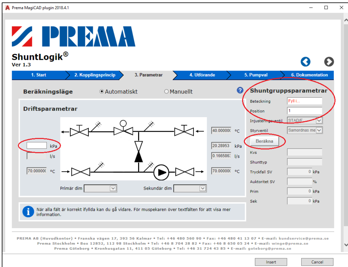
Figure 7 Premablock parameter selection and calculation
