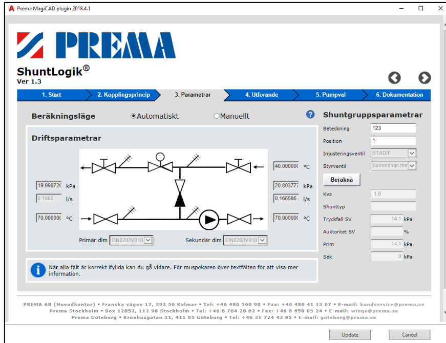
Figure 15 Shunt update operation in parameters
