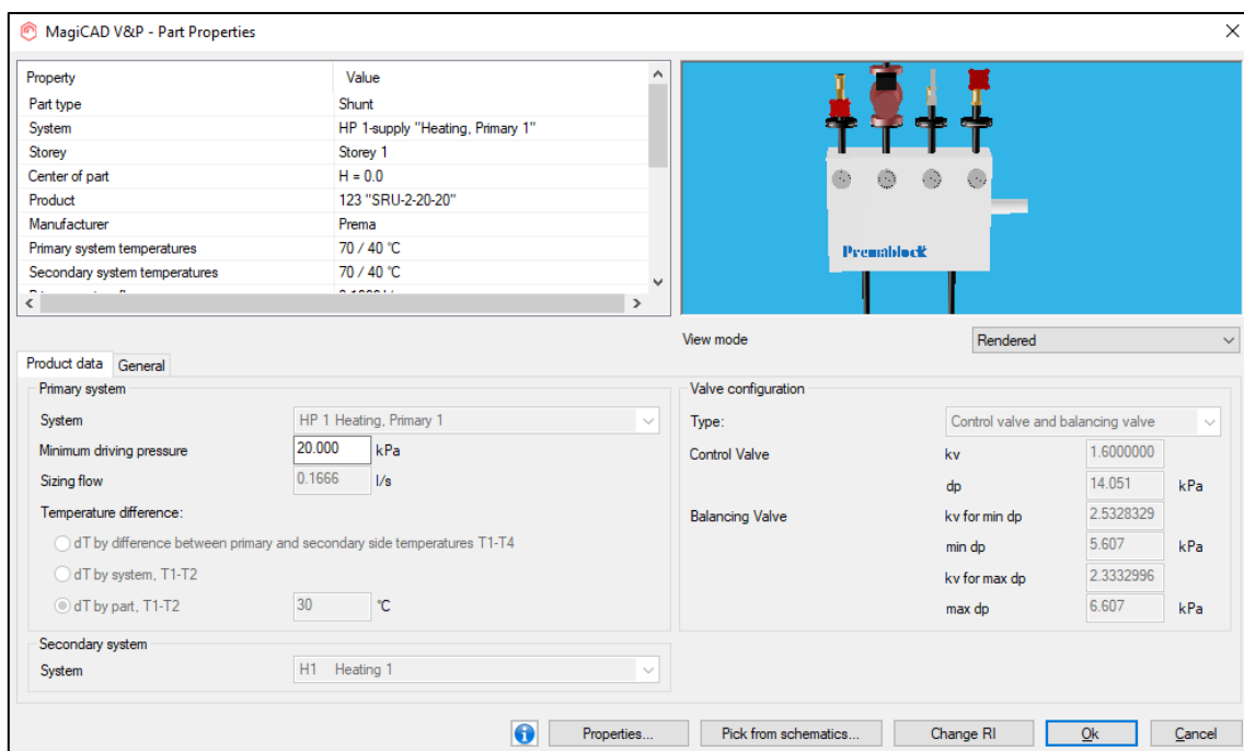
Figure 10 Shunt part properties dialog in MagiCAD
