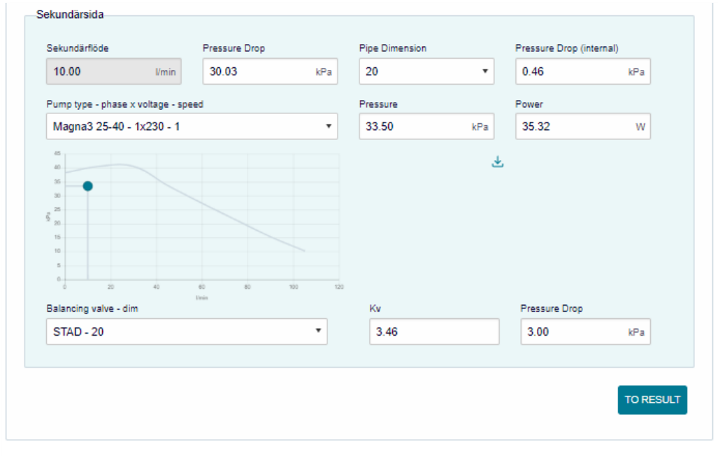
Figure 21 Calculation result page in shunt sizing application
