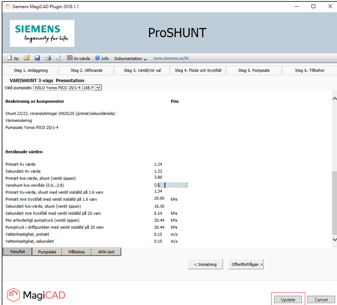
Figure 28 Inserting updated VARISHUNT unit in to MagiCAD
