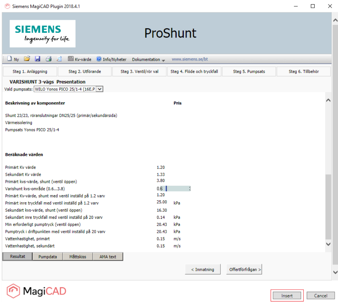
Figure 10 Shunt dimension results page and insert shunt to the MagiCAD project and AutoCAD drawing
