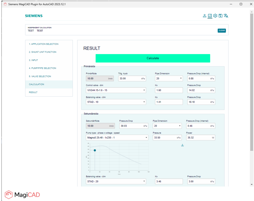
Figure 20 Step 6/6 - Shunt calculation and result page
