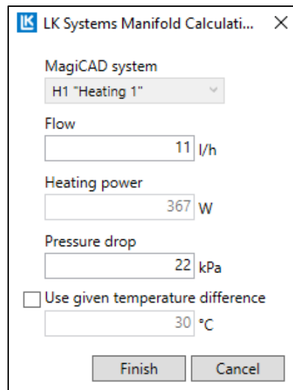
Figure 8 LK Systems floor heating manifolds calculation data dialog
