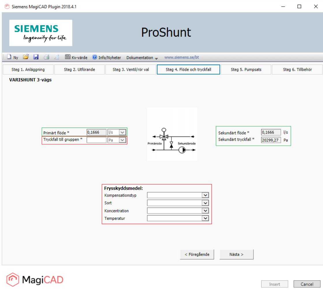
Figure 7 Step 4/6 - Shunt flow, pressure and refrigerant selections
